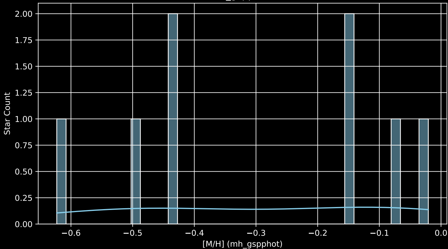
GALAH DR4 Field: [7368] [M/H] (mh_gspphot) (n= 8)
