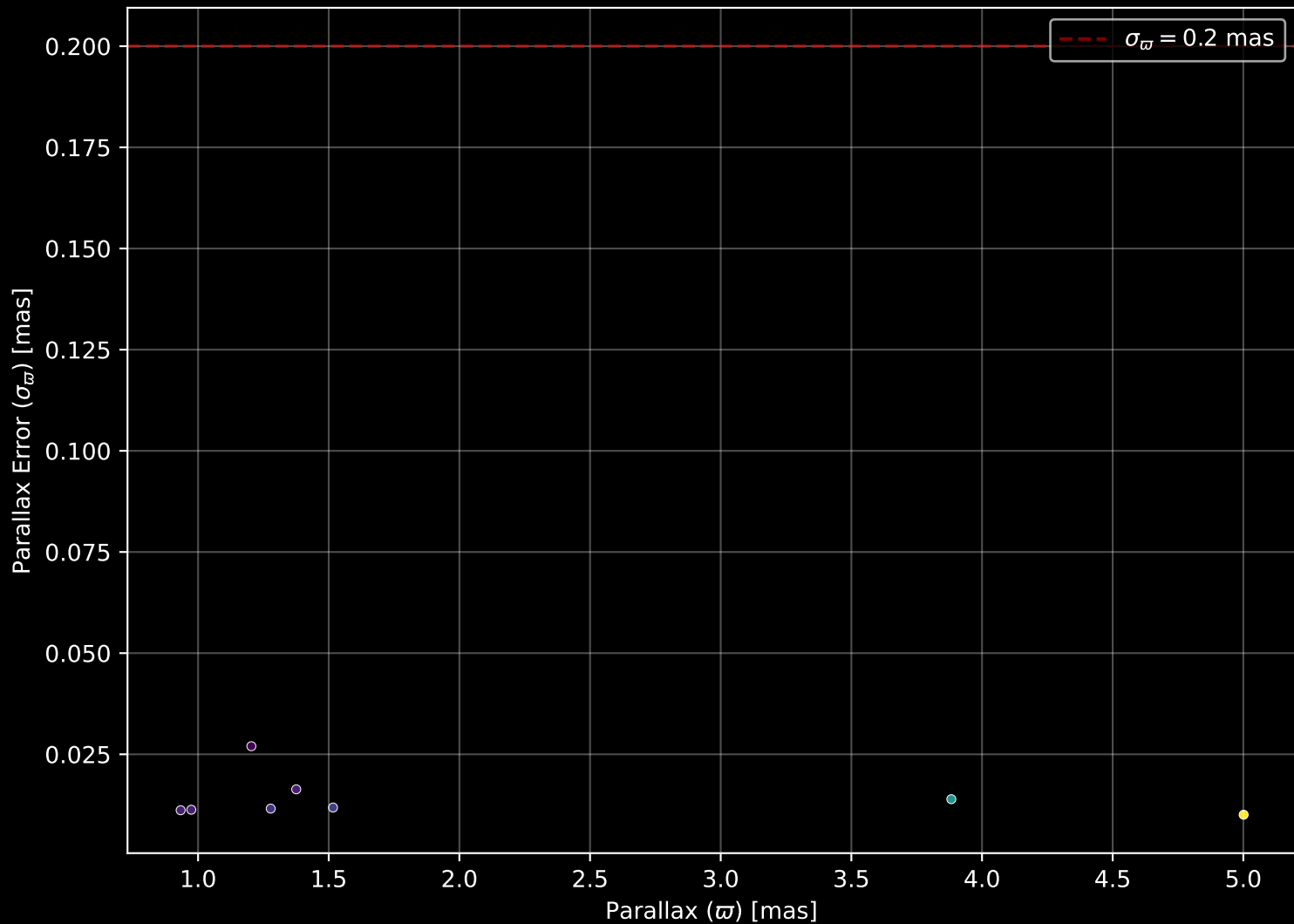
GALAH DR4 Field: [7368] Parallax Quality (n= 8)
