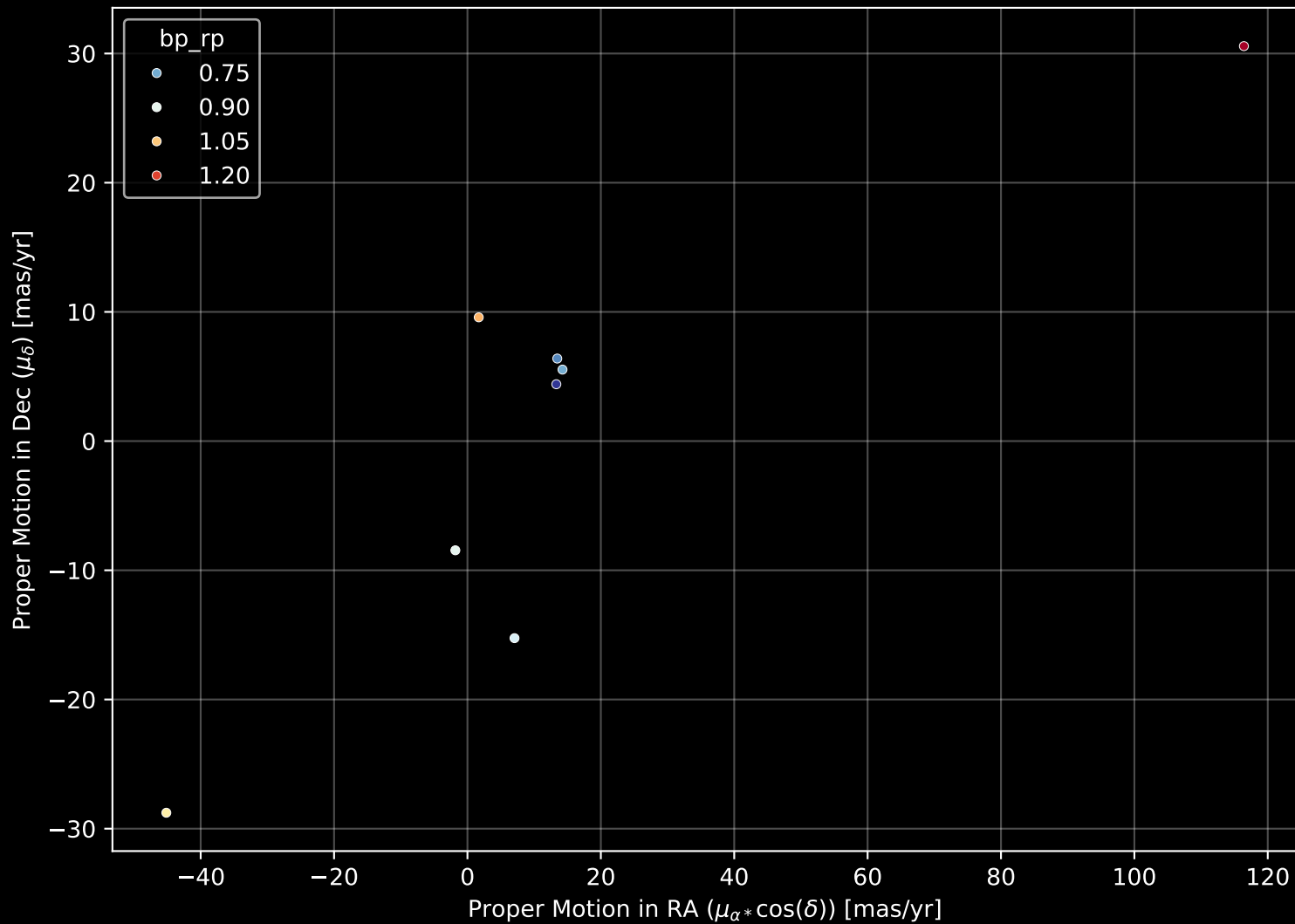
GALAH DR4 Field: [7368] Proper Motion Diagram (n= 8)
