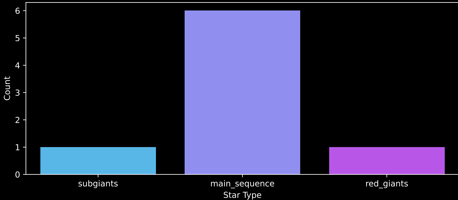
GALAH DR4 Field: [7368] Count plot of Star Type
