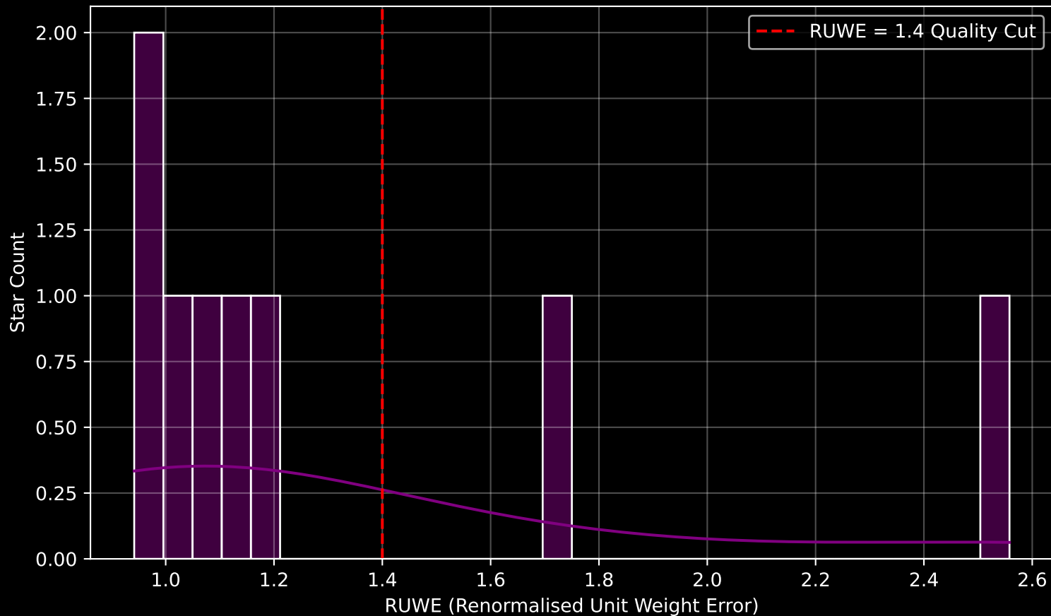
GALAH DR4 Field [7368] RUWE Distribution (n= 8)
